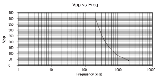
Figure 3: Maximum Vpp vs. Frequency Amplifier's maximum peak-to-peak output roll off with frequency. This is due to the amplifier's slew rate of 250 V/ \mu Sec.
