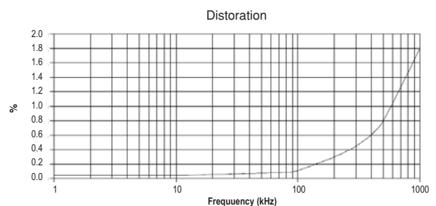
Figure 4: Distortion (Typical) Distortion measurements were made operating the amplifier at 75 % of the maximum Vpp output obtained from Figure 3.
