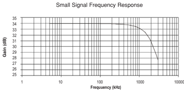
Figure 1: Small Signal Frequency Response (Typical) Amplifier Gain measured with 900 mV peak-to-peak input. Amplifier Frequency Response (-3 dB) at 2 MHz.
