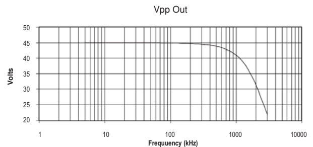
Figure 2: Small Signal Frequency Response (Typical) Amplifier Gain measured with 900 mV peak-to-peak input. Same as Figure 1 but Y-axis is Volts instead of dB.
